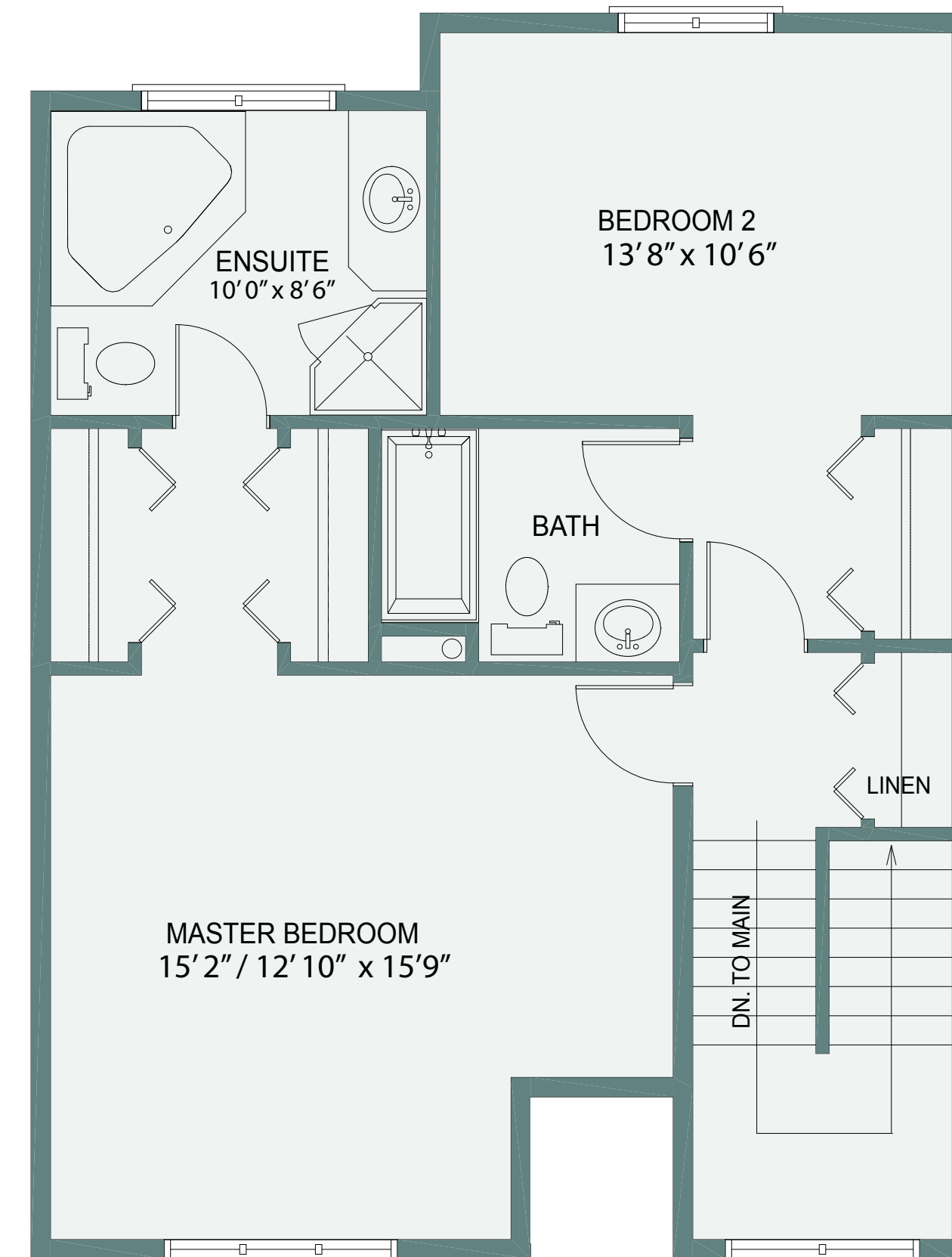
UPPER LEVEL PLAN 662 SQ. FT.
