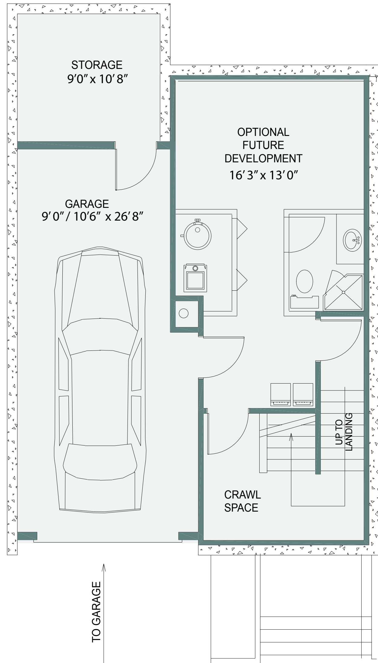
LOWER LEVEL PLAN
