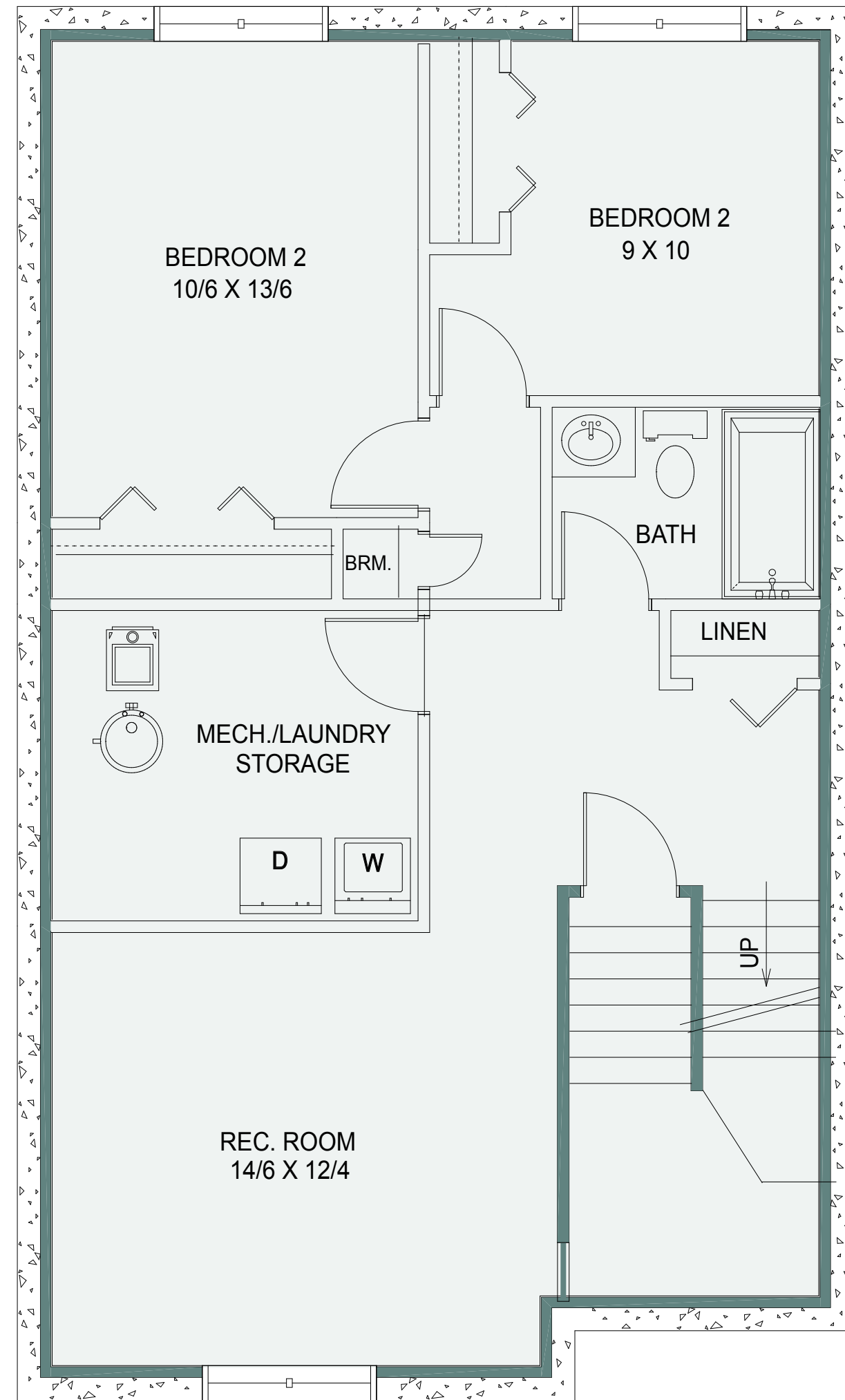
OPTIONAL LOWER DEVELOPMENT PLAN 944 SQ. FT.
